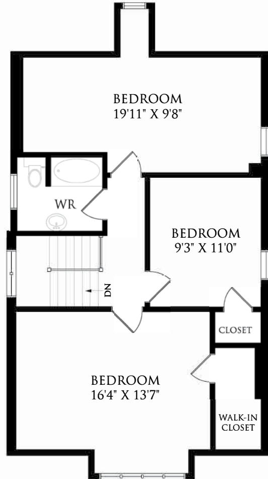
THIRD FLOOR 780 SQUARE FEET
