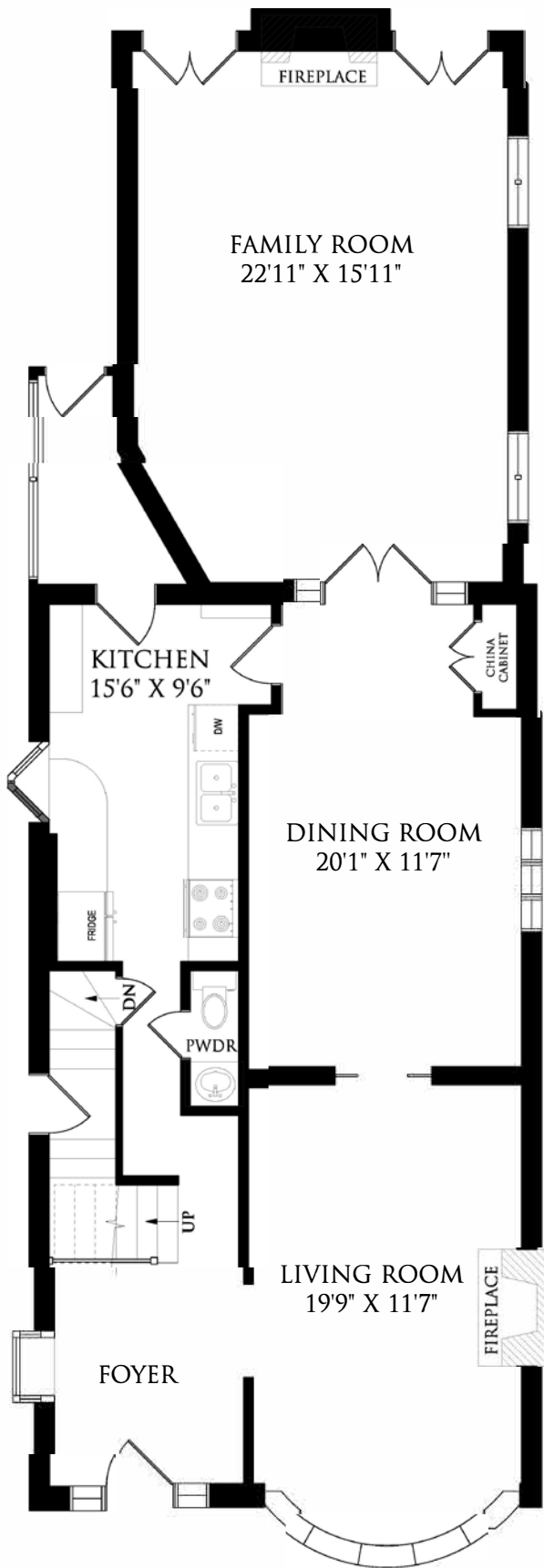
MAIN FLOOR 1310 SQUARE FEET
