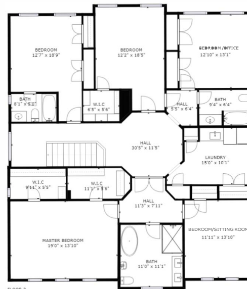
FLOOR 3
