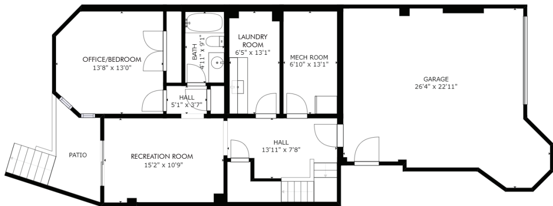
LOWER LEVEL
