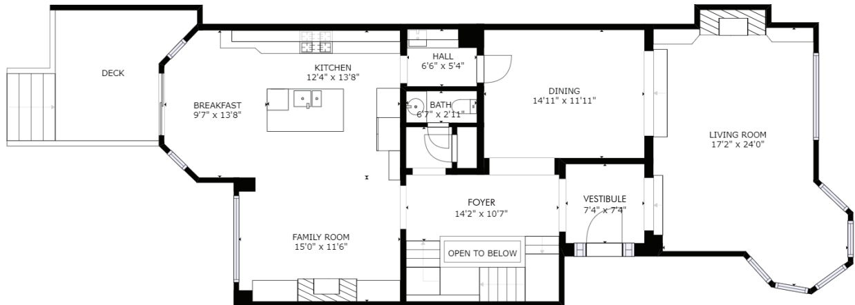
MAIN FLOOR
