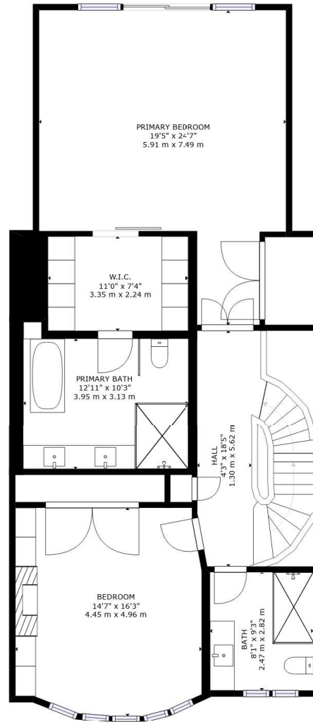
FLOOR 3
