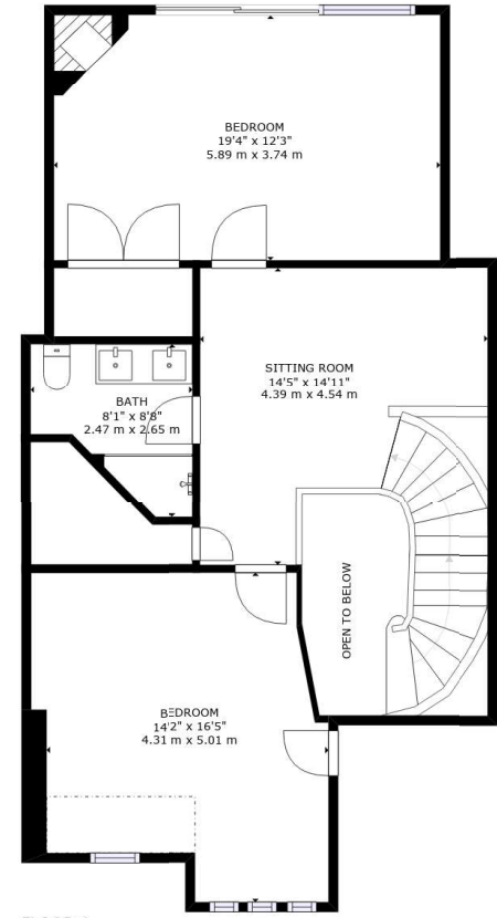
FLOOR 4
