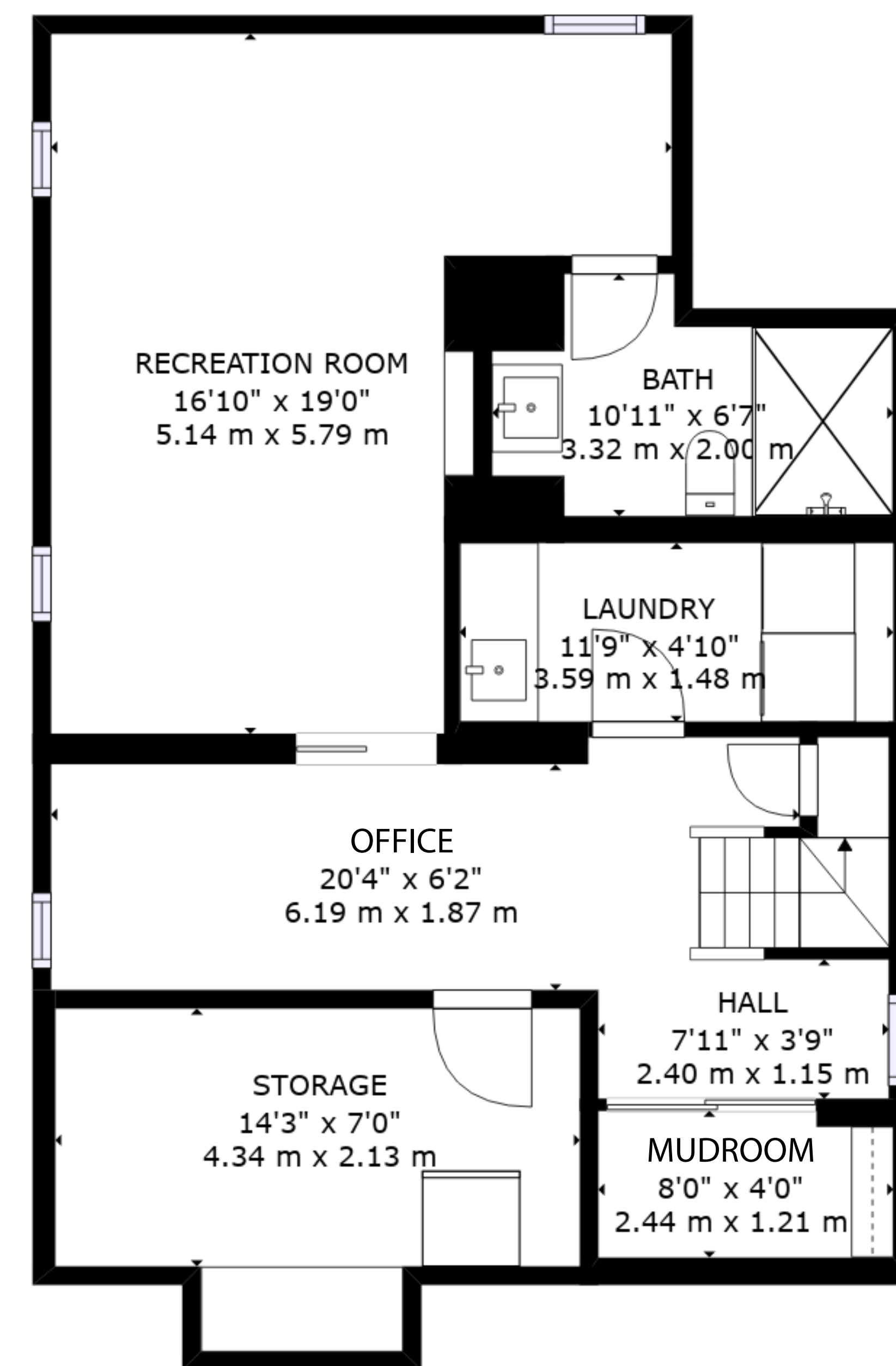
LOWER LEVEL
